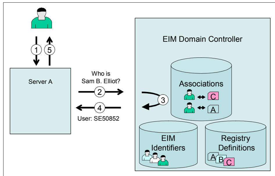
Figure 13-2 EIM flow
