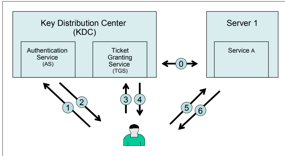
Figure 12-3 Kerberos flow
