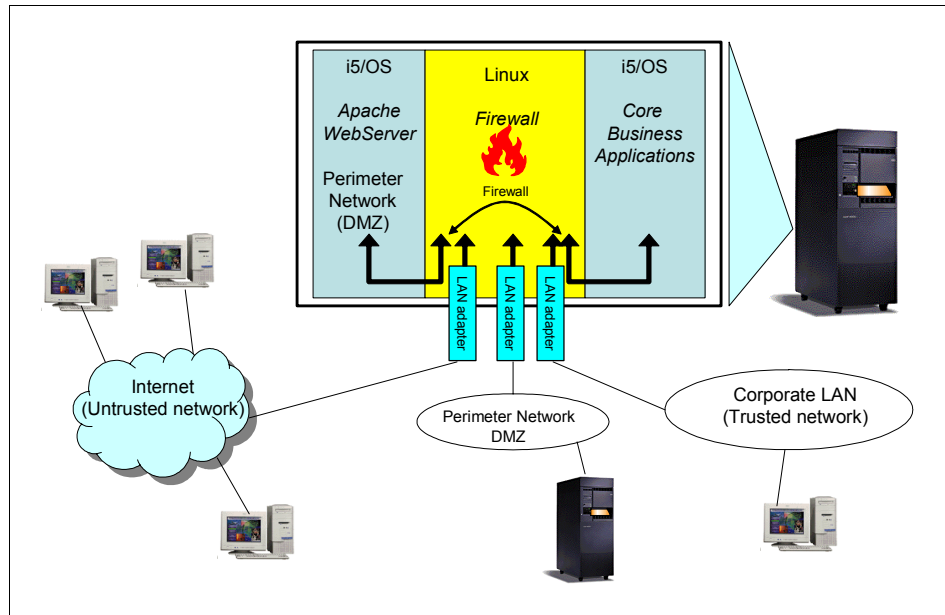
Figure 11-7 System i machine protected by one firewall
