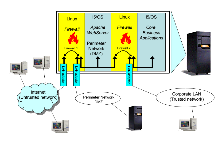
Figure 11-6 i5/OS partitions under control of the firewall
