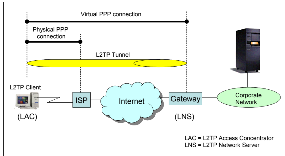
Figure 10-5 L2TP voluntary tunnel
