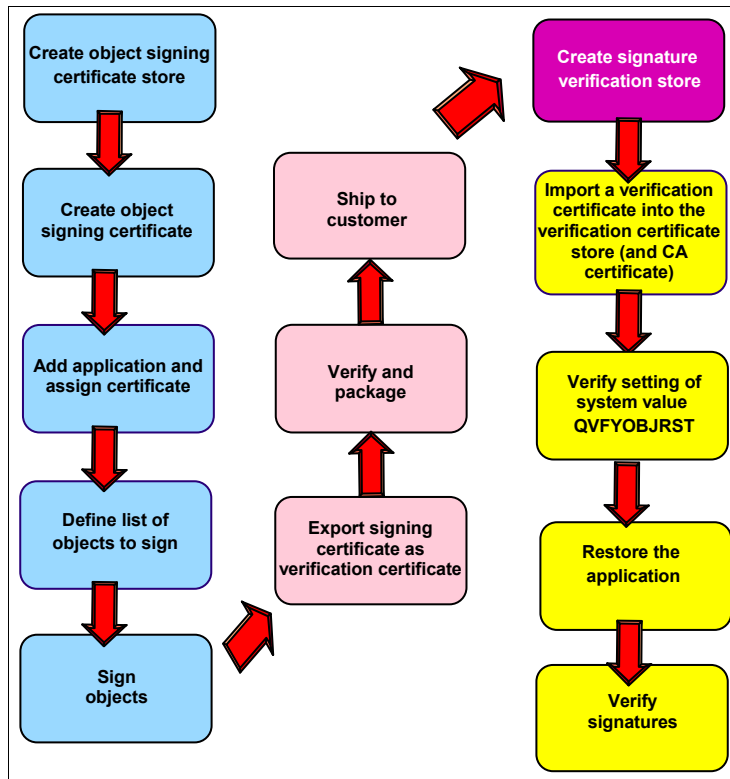
Figure 7-2 Overview of object signing
