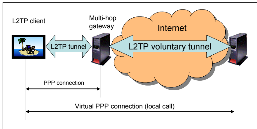
Figure 10-6 L2TP multi-hop connection
