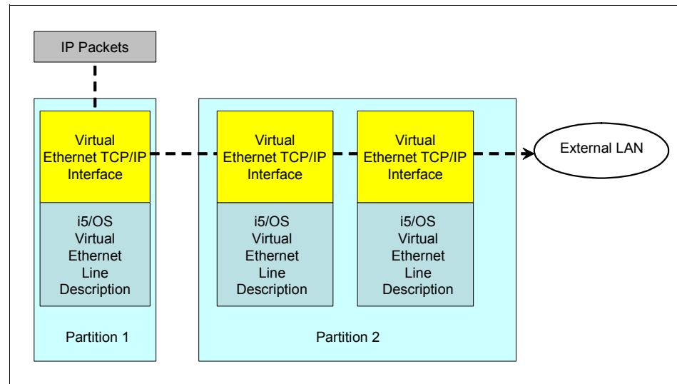
Figure A-8 Connecting virtual Ethernet to external LANs
