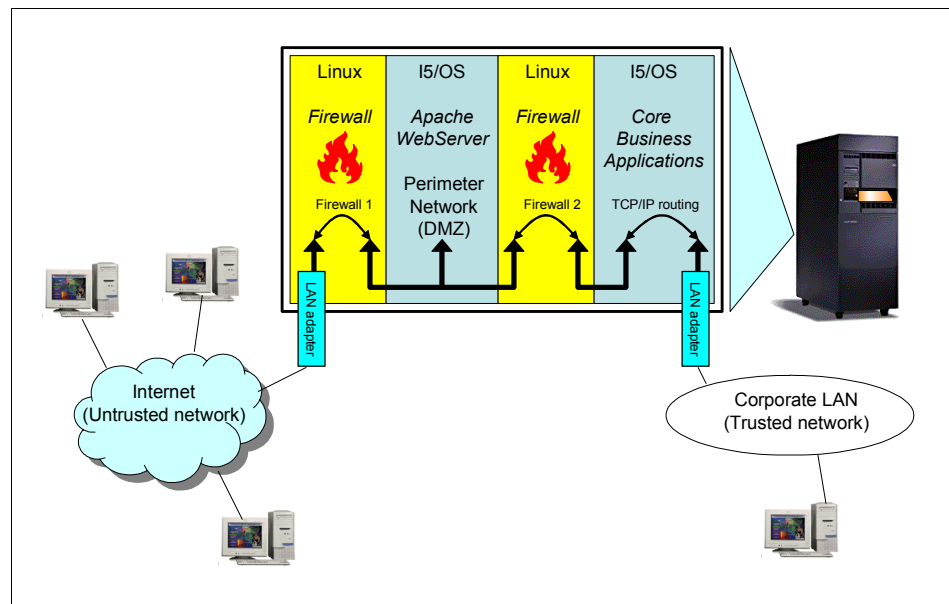
Figure 11-4 Scenario using two Linux partitions to create a DMZ
