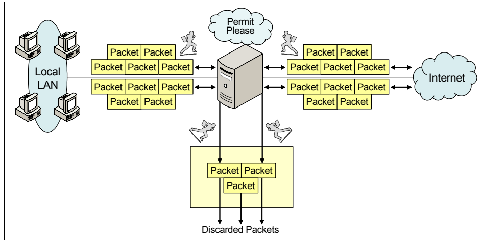
Figure 8-13 IP packet filtering principles
