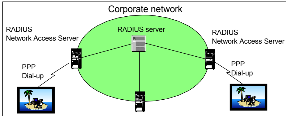
Figure 8-18 Authentication with a RADIUS server
