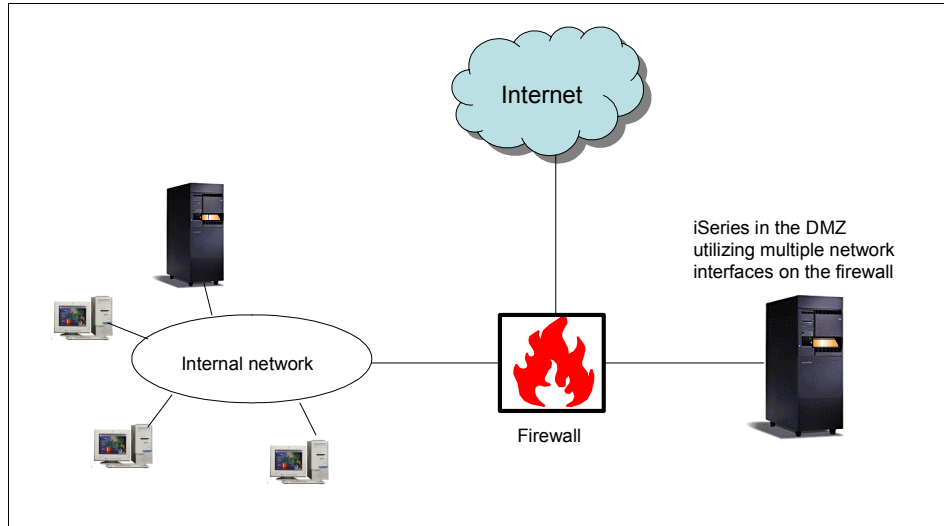
Figure 11-3 Single firewall solution or three-legged firewall solution
