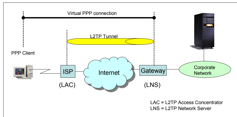
Figure 10-4 L2TP compulsory tunnel
