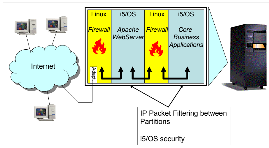
Figure A-7 Server consolidation
