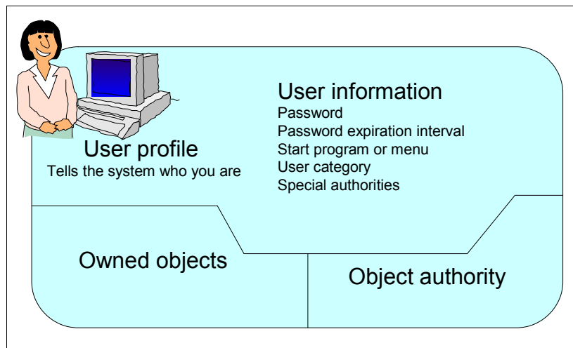
Figure 4-2 User profile
