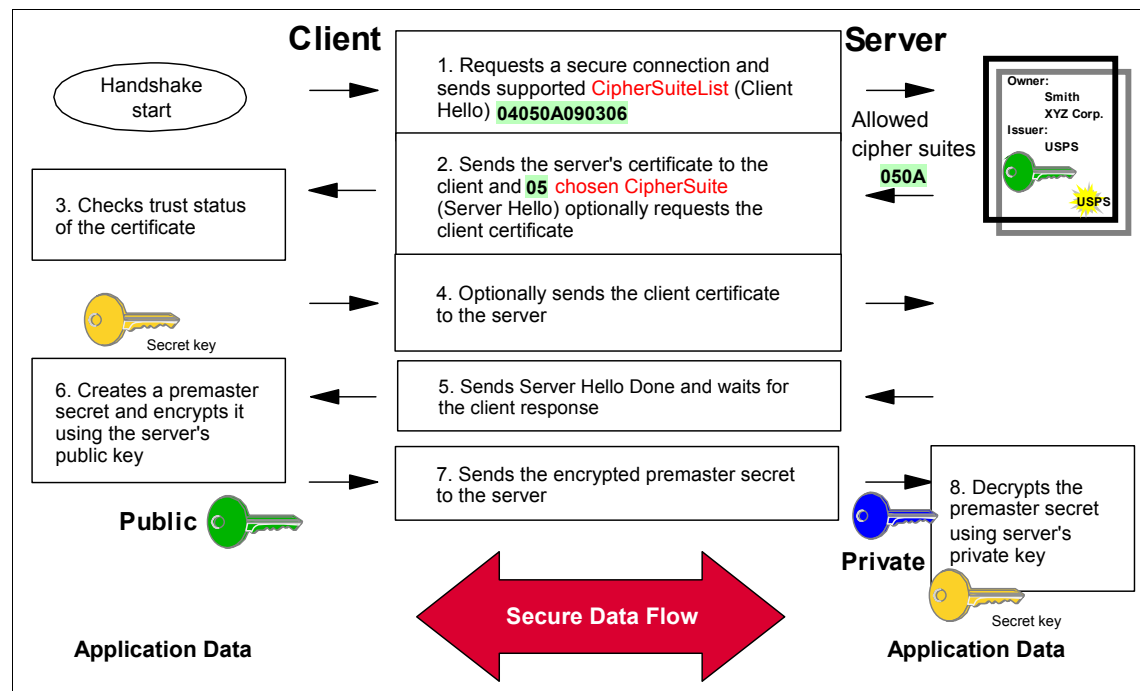
Figure 9-9 SSL handshake
