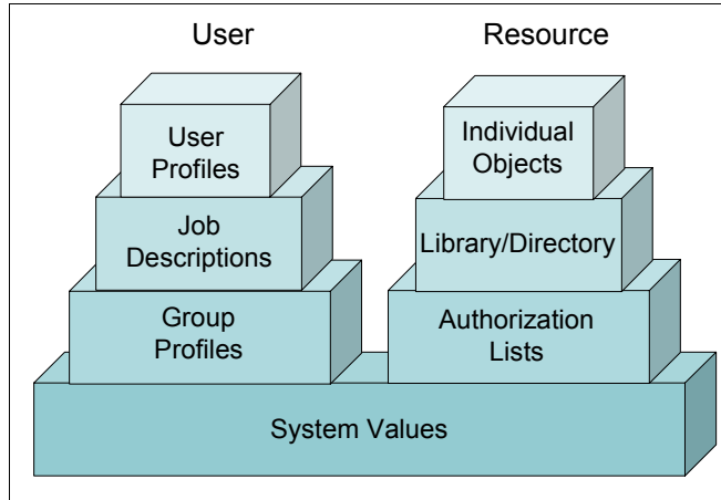
Figure 4-1 Security components
