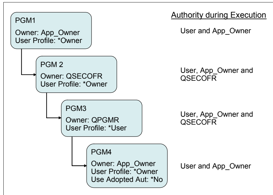
Figure 4-5 Adopted authority
