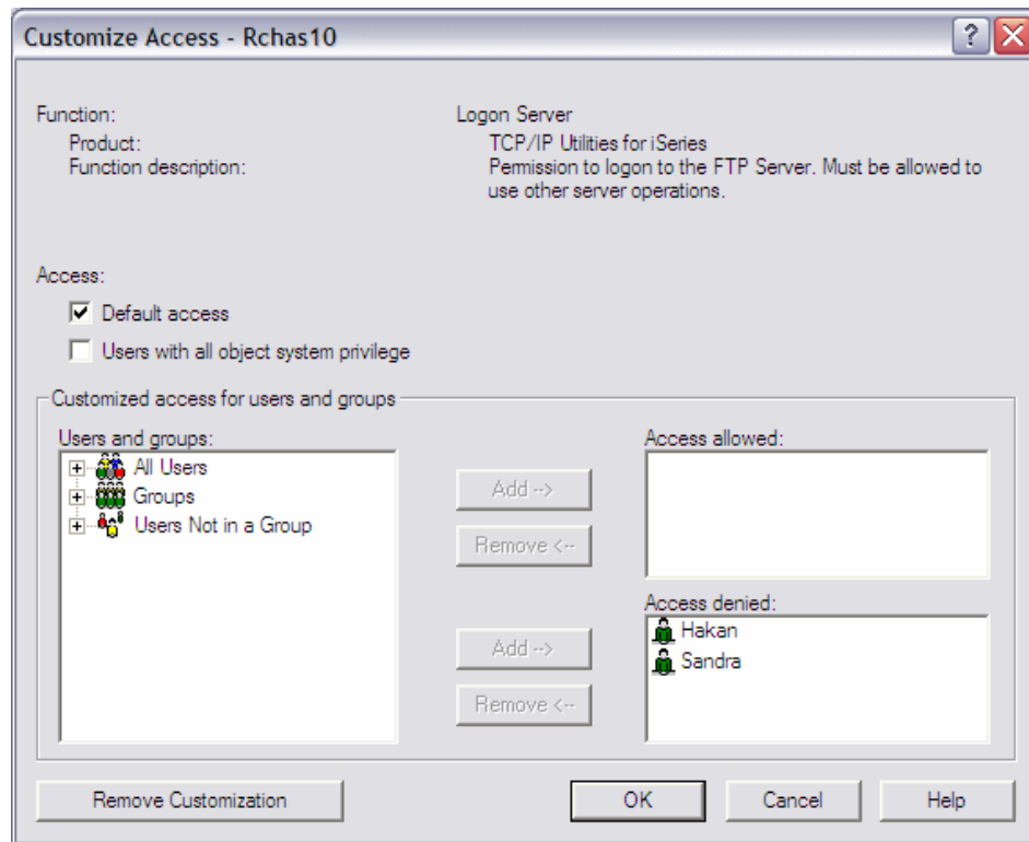
Figure 4-13 Customize Access
