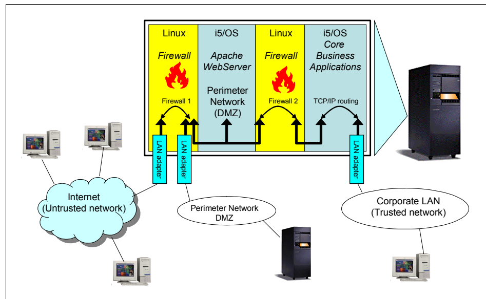
Figure 11-5 DMZ for other hosts
