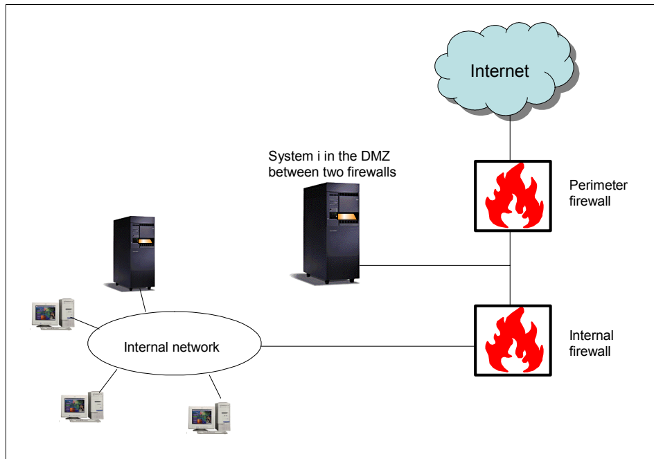
Figure 11-2 Dual firewall with a DMZ between
