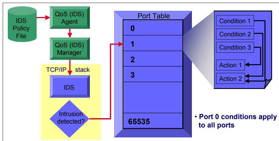
Figure 8-17 i5/OS IDS implementation overview
