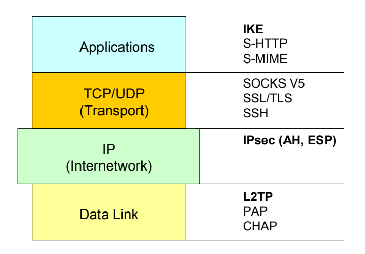
Figure 10-2 TCP/IP protocol stack with VPN-related protocols
