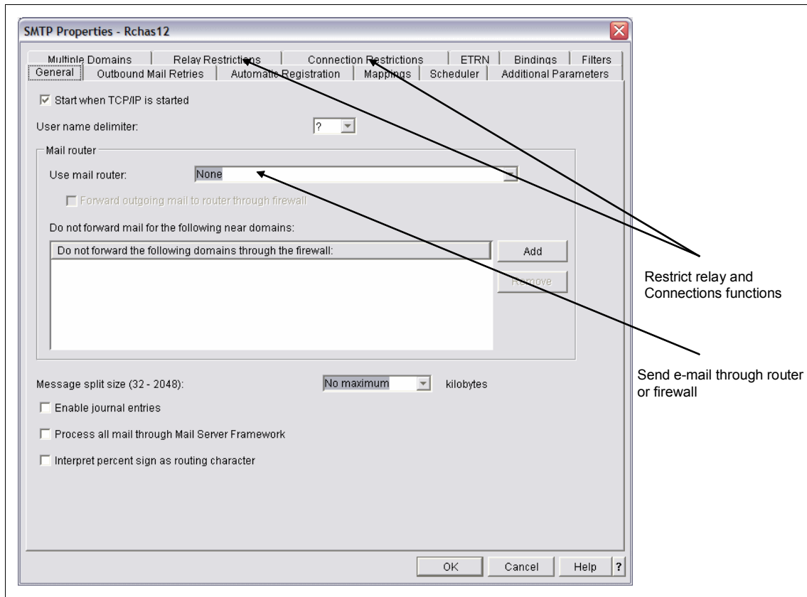
Figure 8-23 SMTP properties
