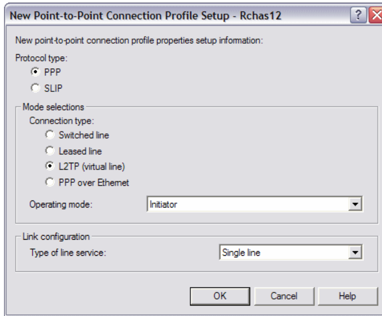
Figure 10-10 PPP configuration
