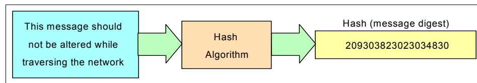
Figure 9-2 Hashing mechanism
