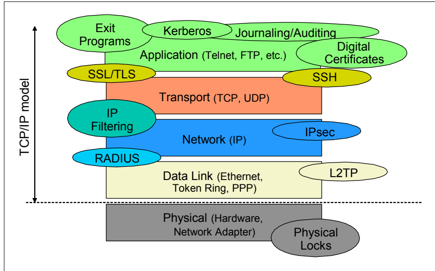
Figure 8-1 TCP/IP model
