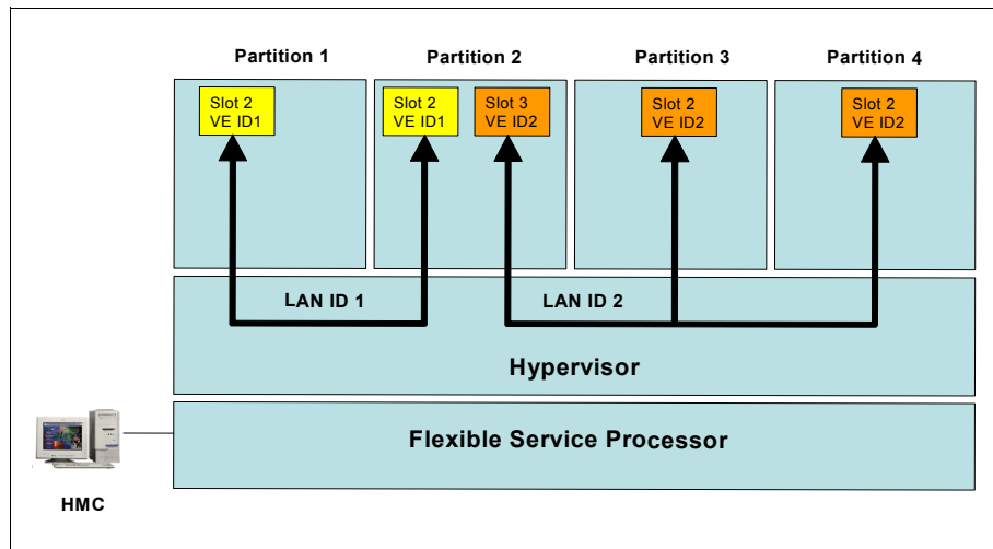
Figure A-6 Virtual Ethernet
